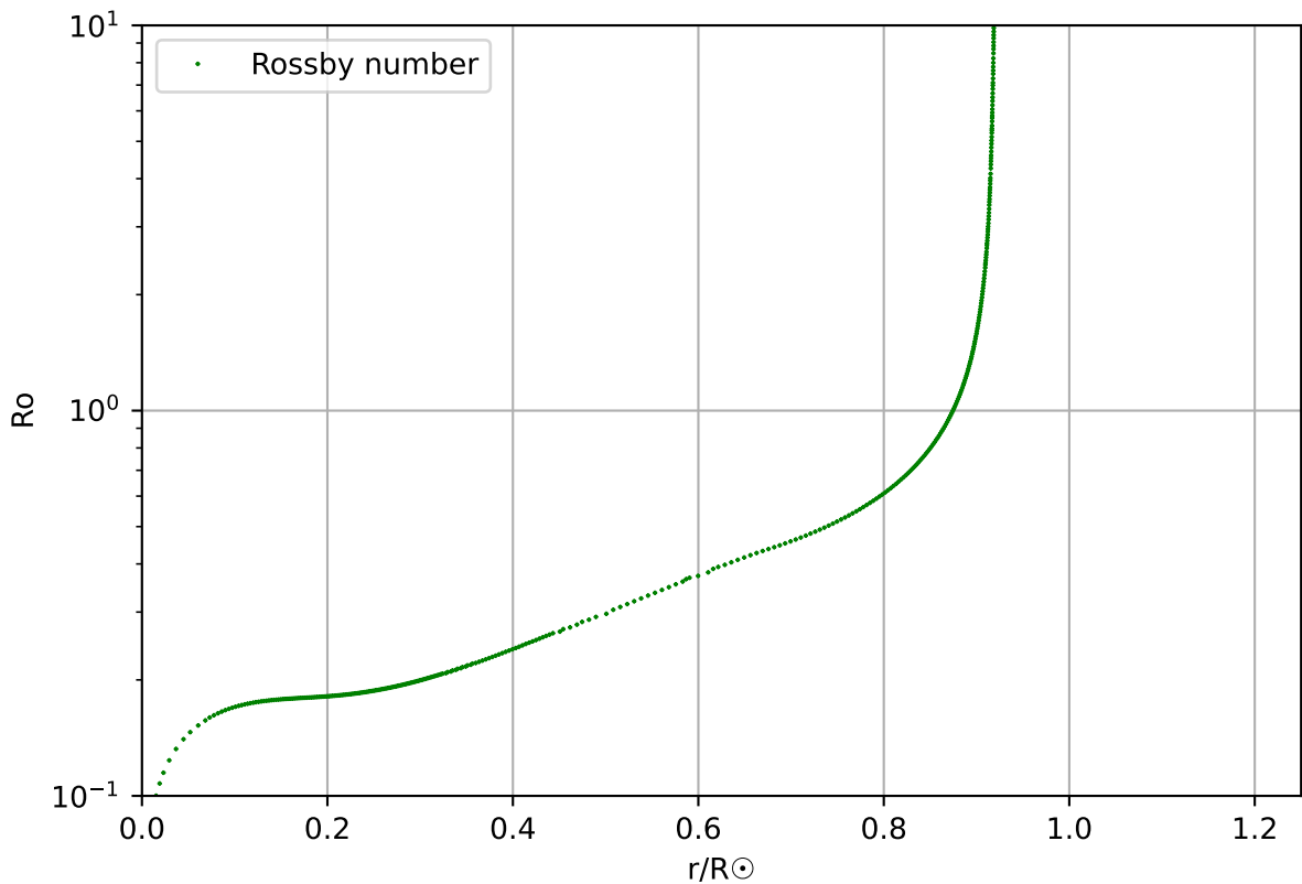
Rossby number, profile 135, age 1.63 \times 10^9
